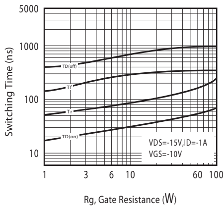
Figure 11. switching characteristics
