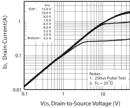
Figure 1. Output Characteristics
